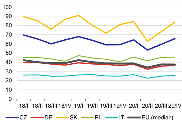
Chart VII.2.3: Goods exports
