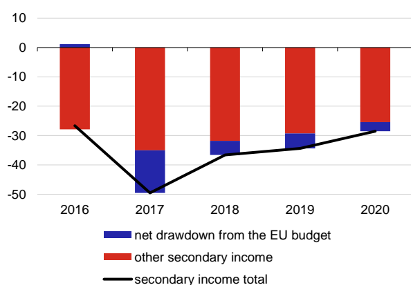
Chart 11: Secondary income
