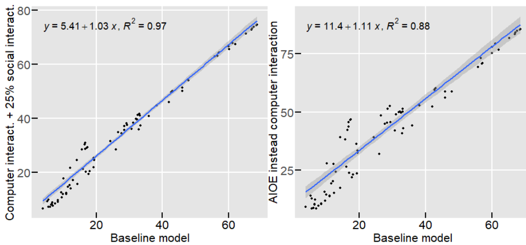
Figure 14: AISA in Comparison to Alternative Models (Computer Interaction Oriented)
