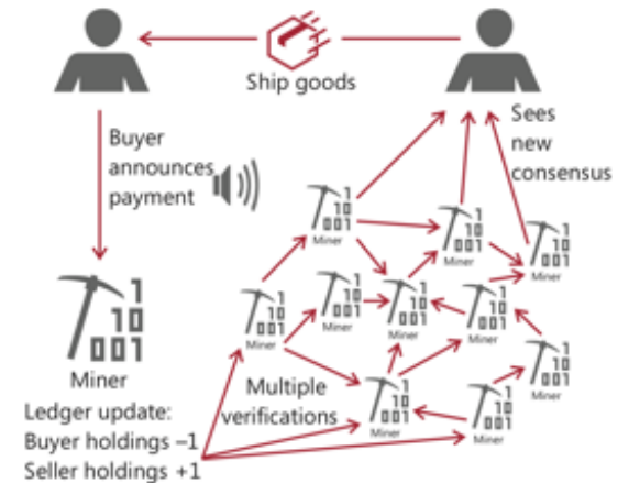
Distributed ledger
