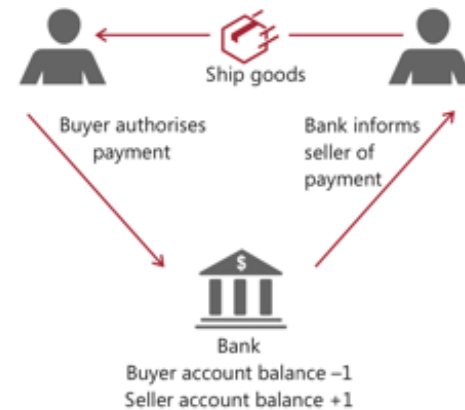
Centralised ledger
