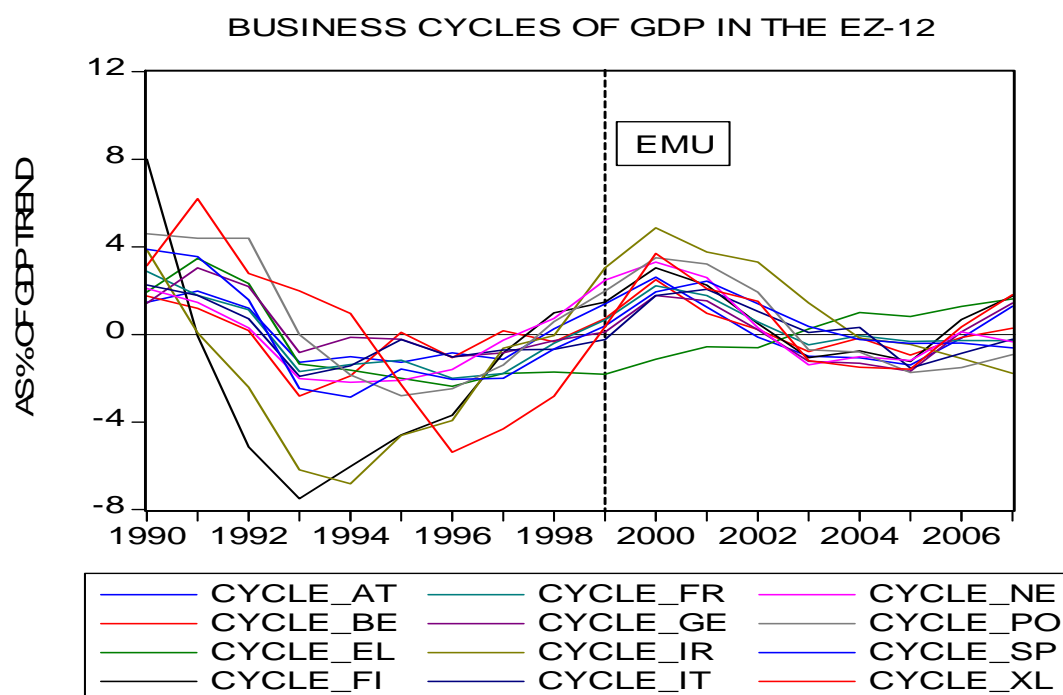
Figure 1a: Per Capita GDP Fluctuations in the Twelve Eurozone Countries (expressed as % of the trend in each country's GDP per capita in constant terms)
