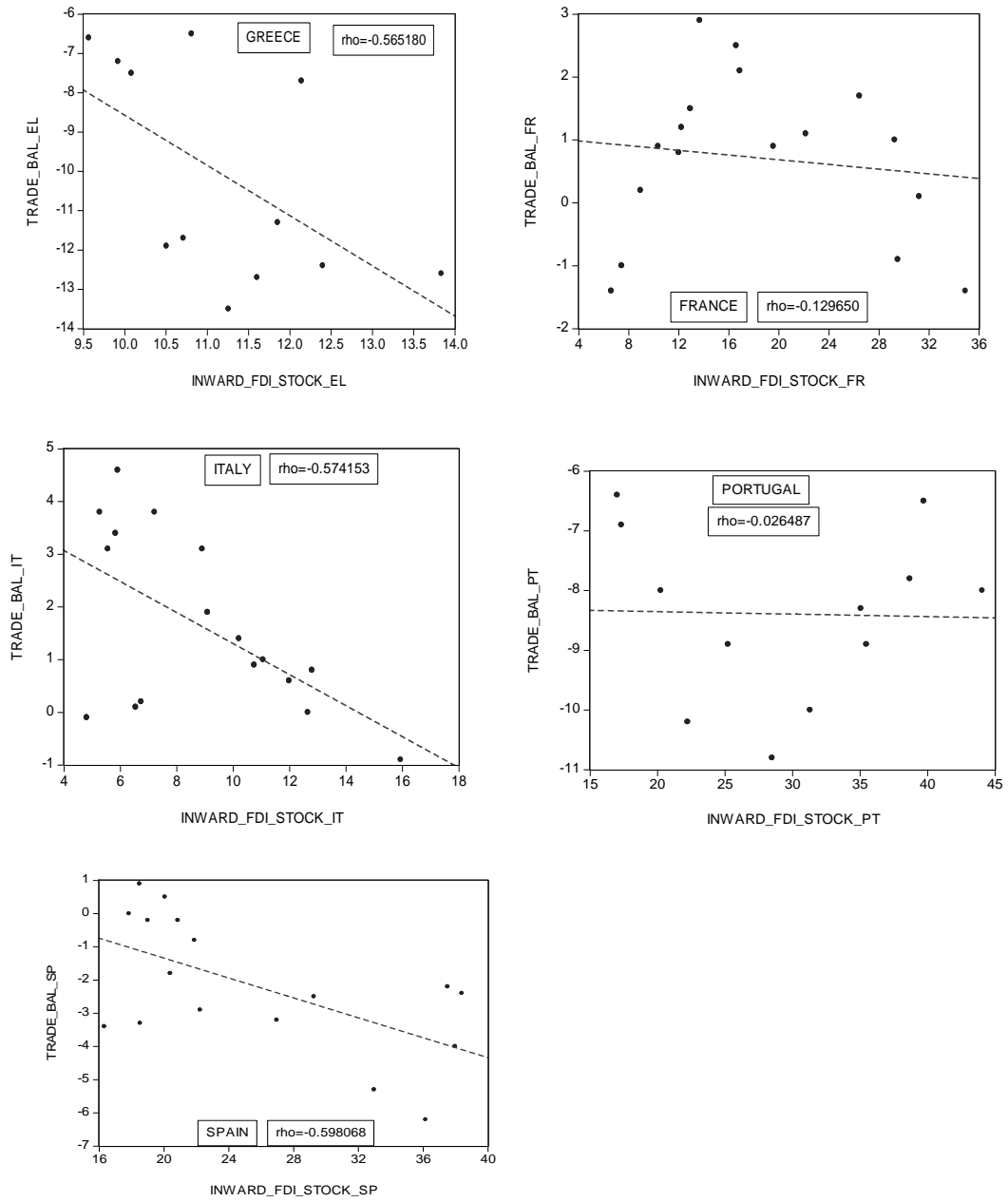
Figure 6b: Correlation between Trade Balances and Inward Investment in the Southern Eurozone Countries 1990–2006
